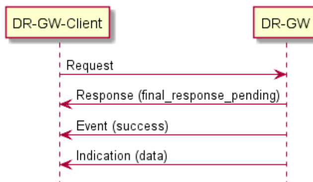
Figure 36 – Successful request/response
