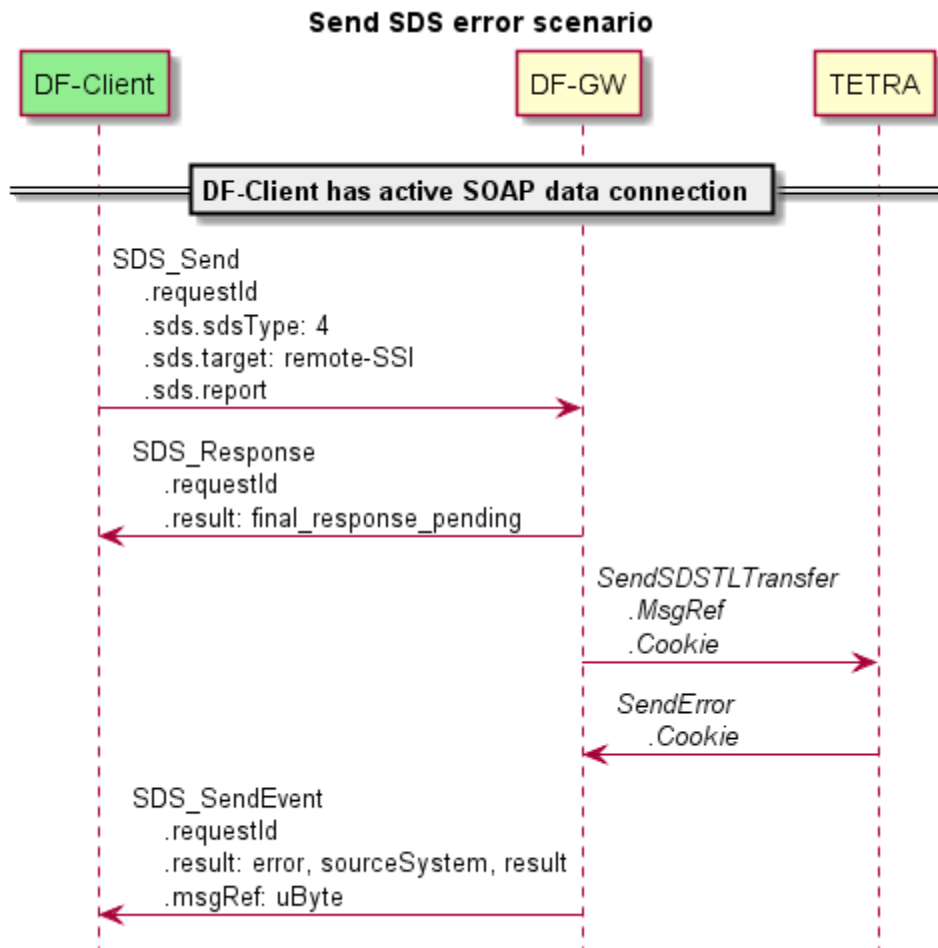
Figure 28 – MSC Send SDS error scenario
