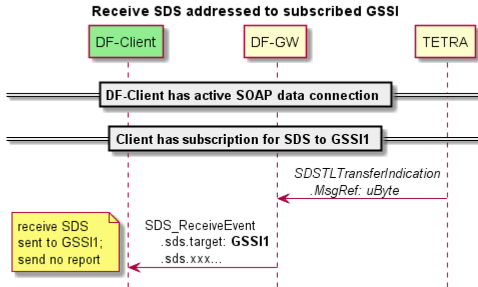
Figure 30 – MSC Receive SDS addressed to subscribed GSSI
