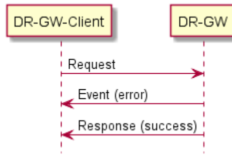
Figure 39 –Asynchronous fired error
