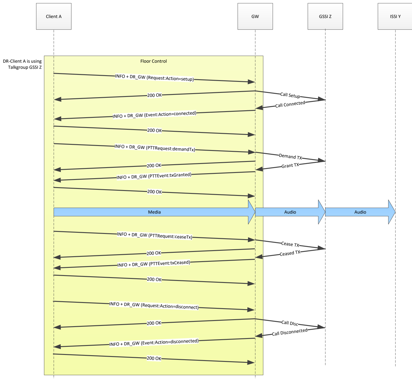
Figure 18 – MSC Floor Life Cycle
