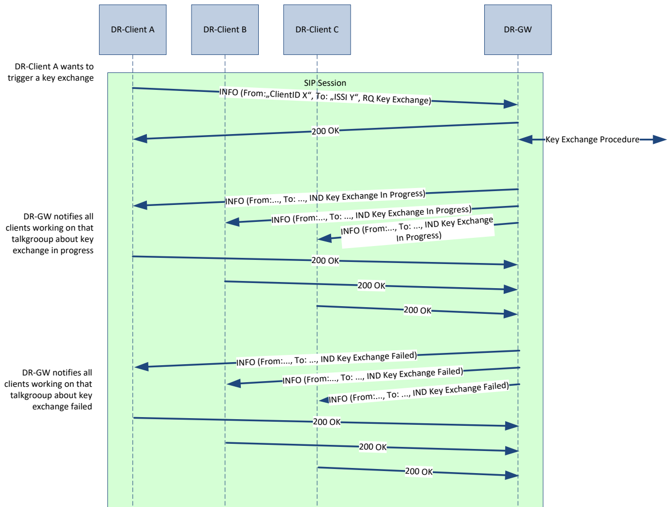
Figure 24 – MSC for unsuccessful new key demand
