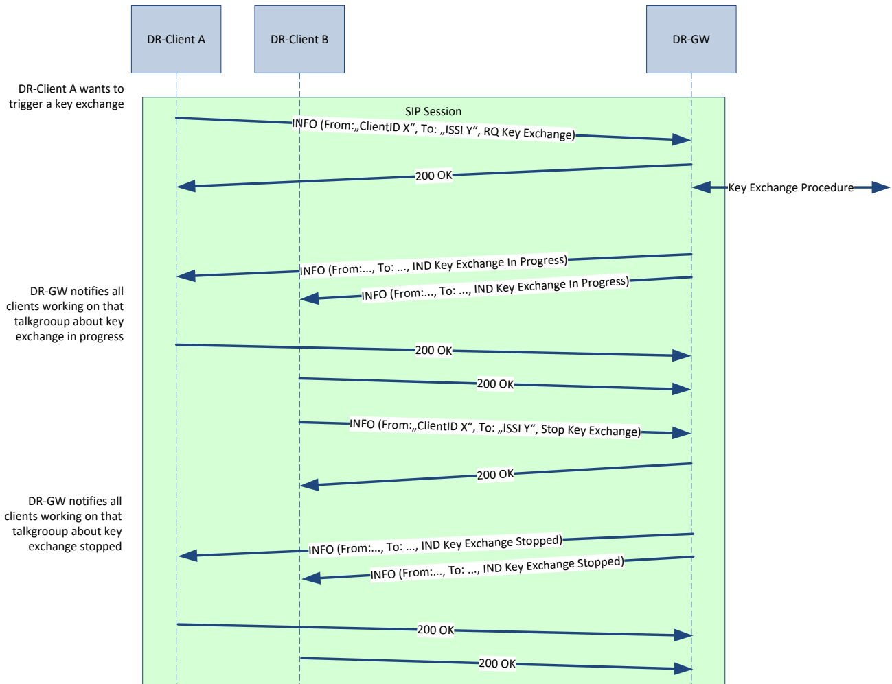
Figure 25 – MSC for client aborting new key demand
