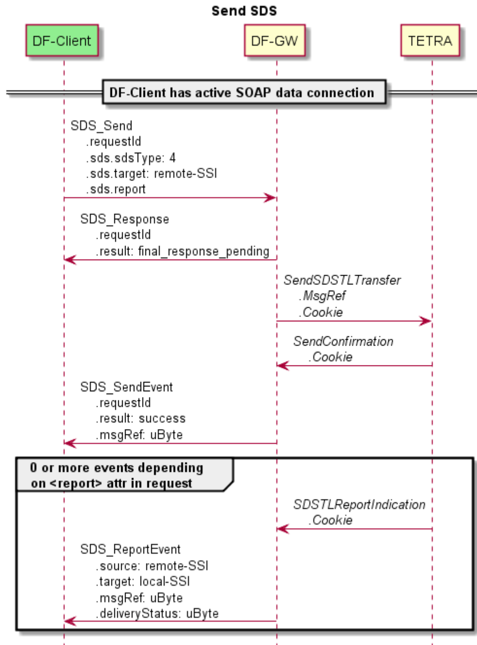
Figure 27 – MSC Send SDS
