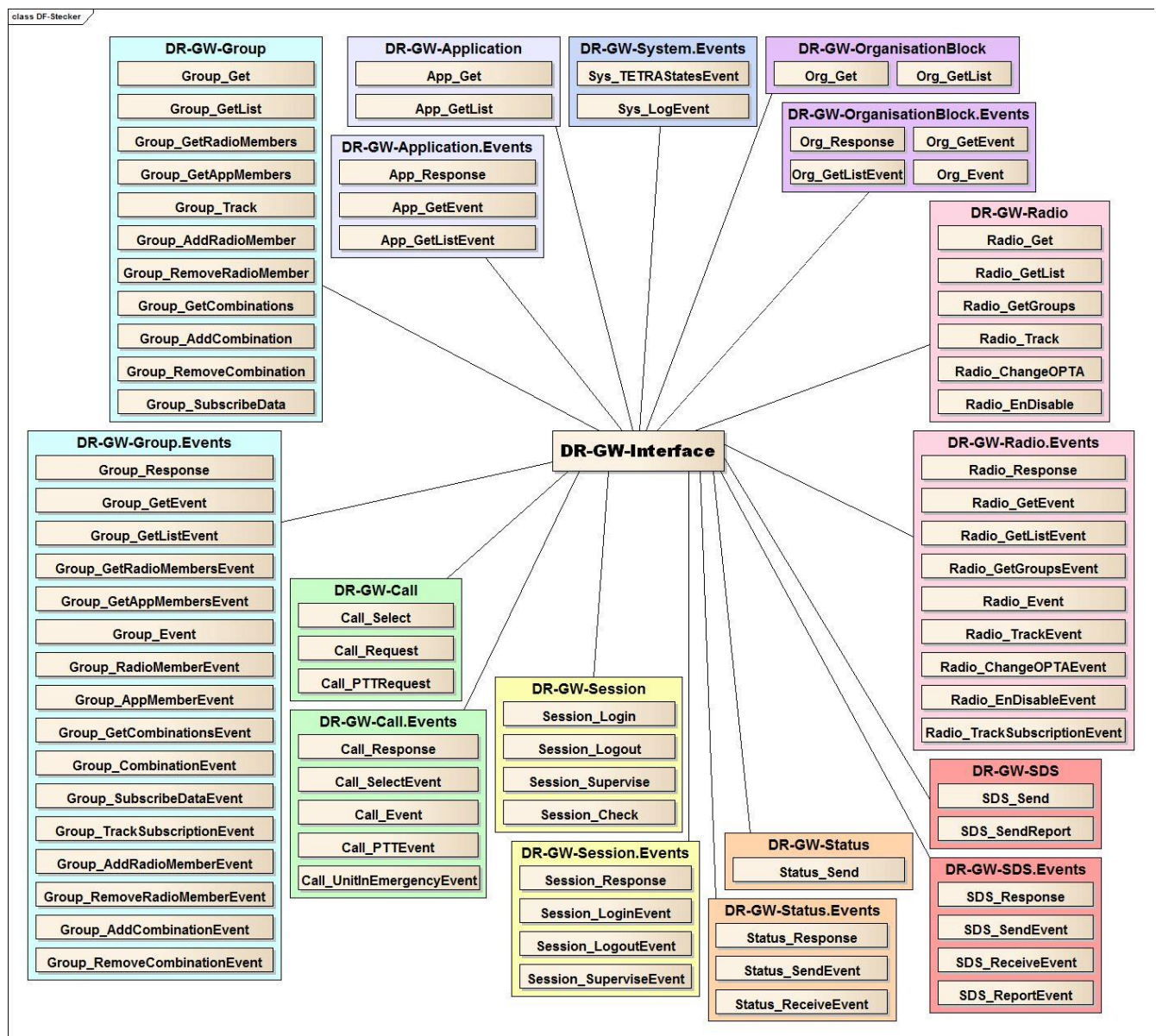
Figure 40 – DR-GW Graph
