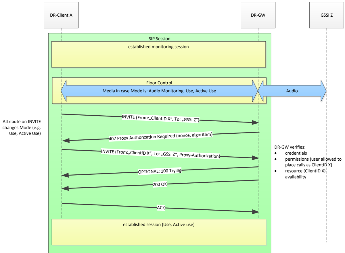
Figure 17 – MSC for GW accepted Selection Mode change
