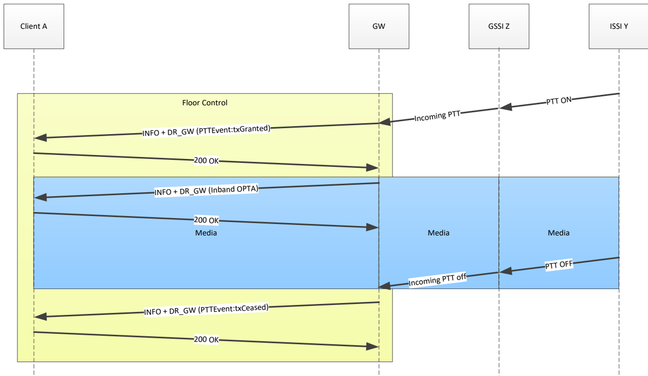
Figure 20 – MSC Floor Control In
