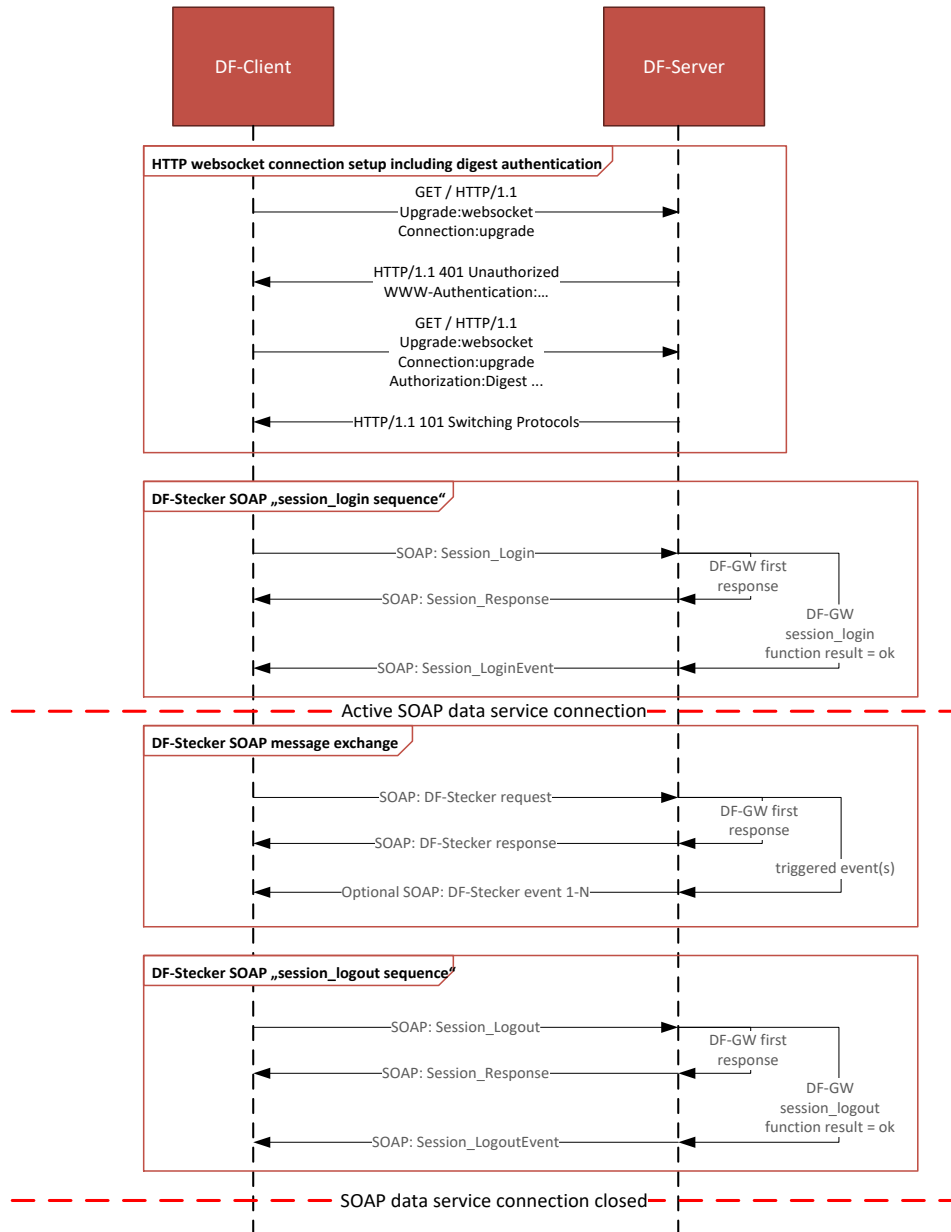
Figure 35 – SOAP Session Life-Cycle
