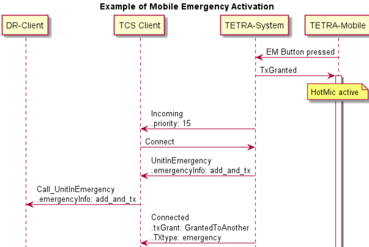
Figure 26 – MSC for Unit in Emergency
