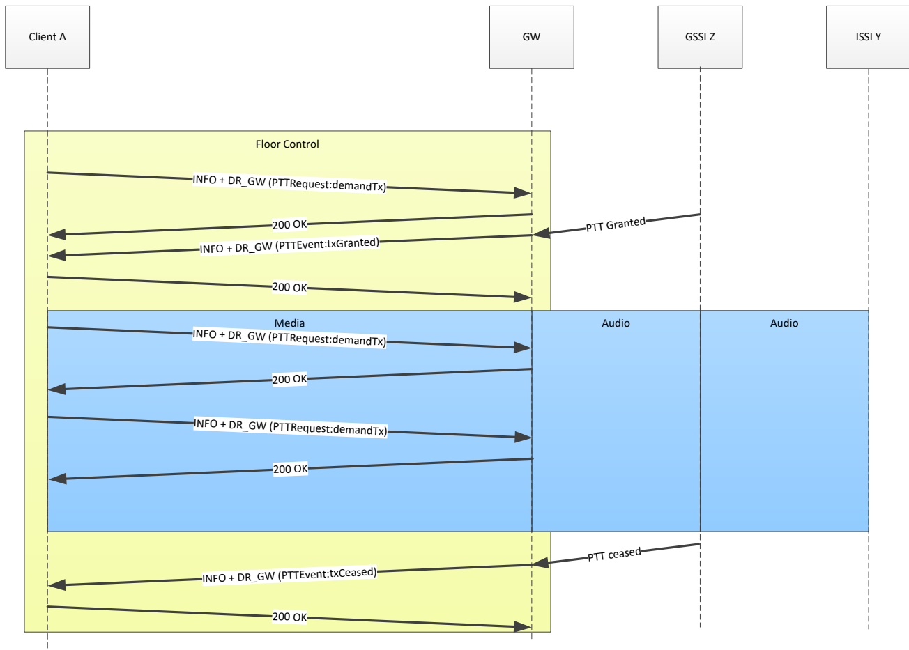
Figure 19 – MSC Floor Control Out
