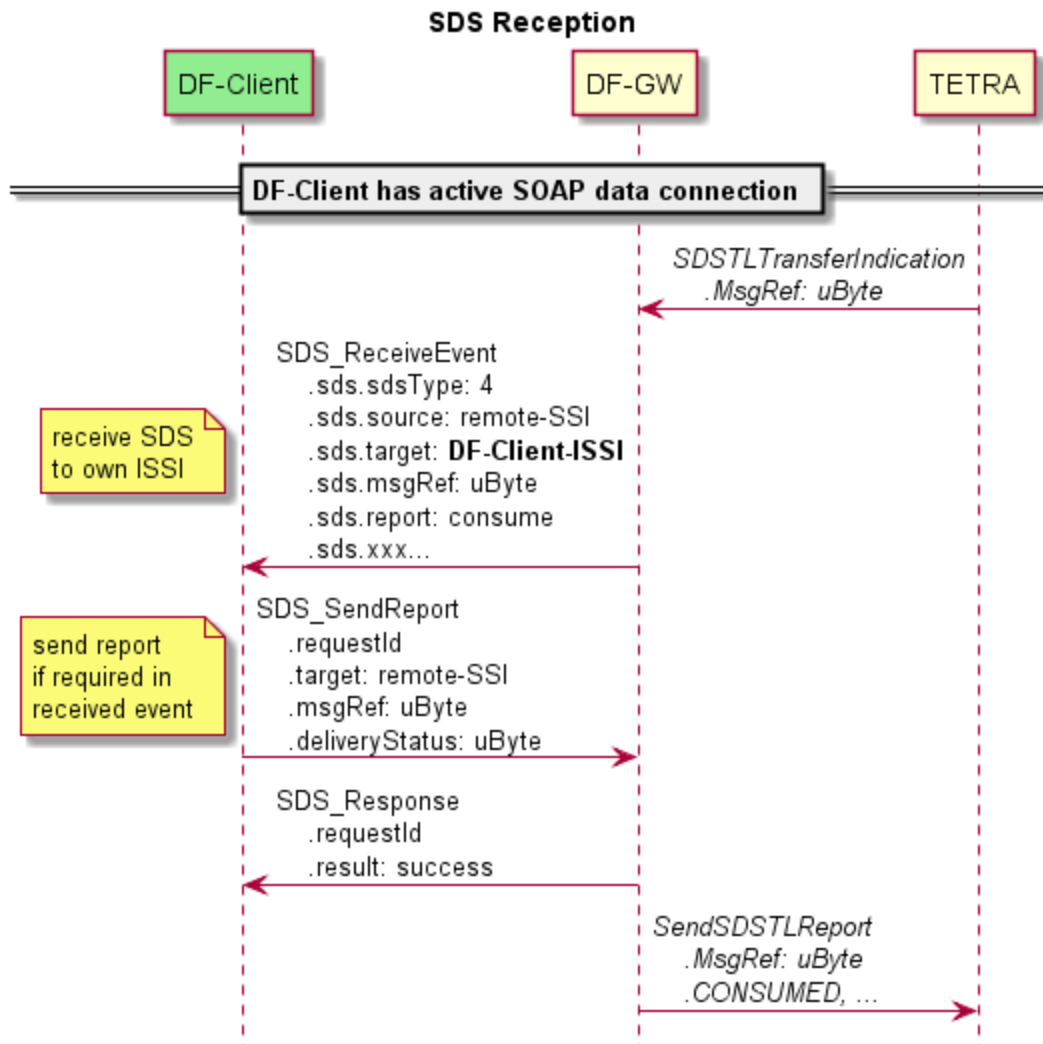
Figure 29 – MSC Receive SDS
