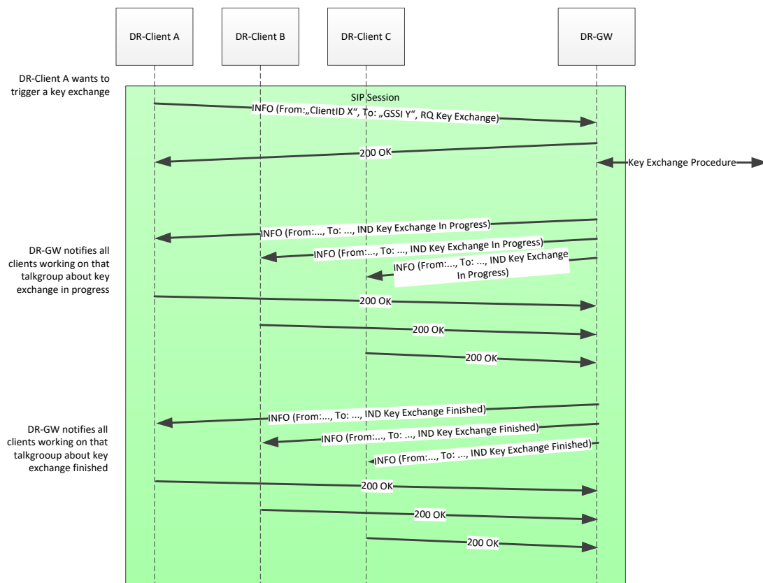
Figure 23 – MSC for DR-GW-Client demanding a new key
