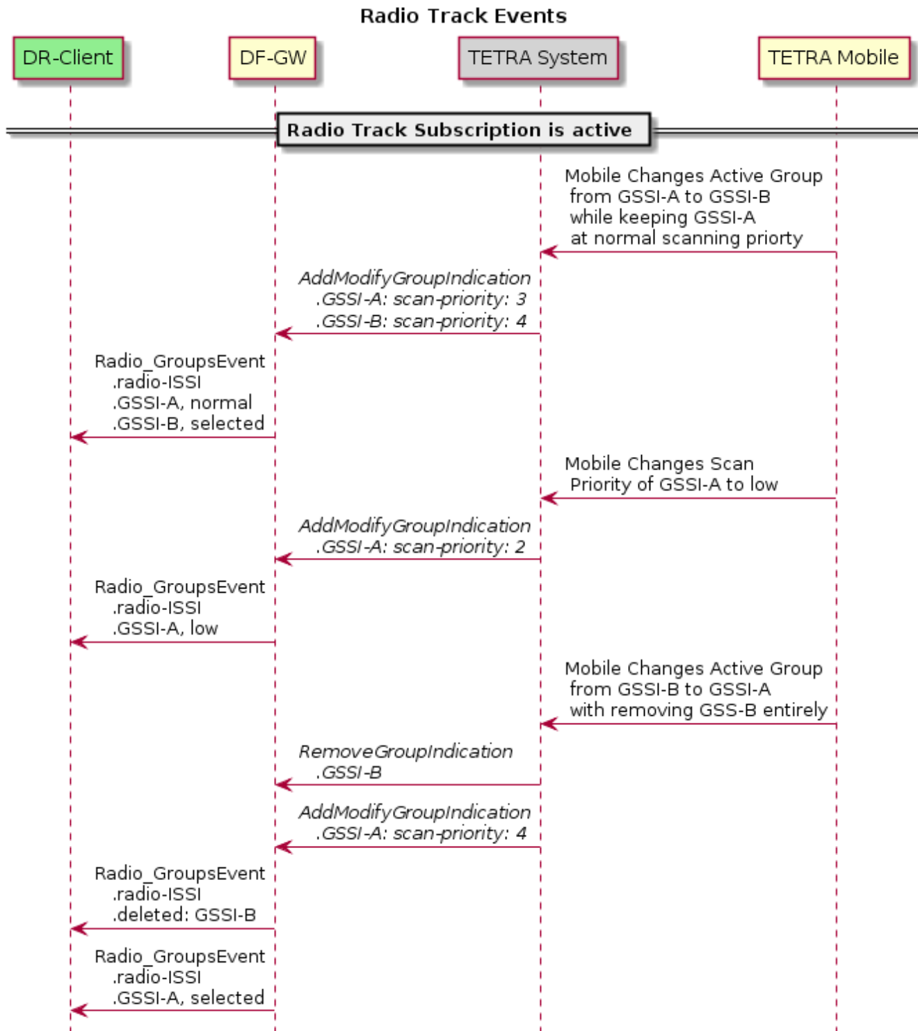
Figure 32 – Radio Track Events
