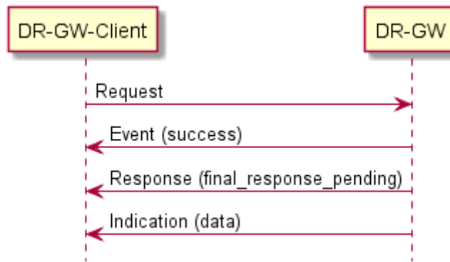
Figure 37 –Request/response with Event before Response
