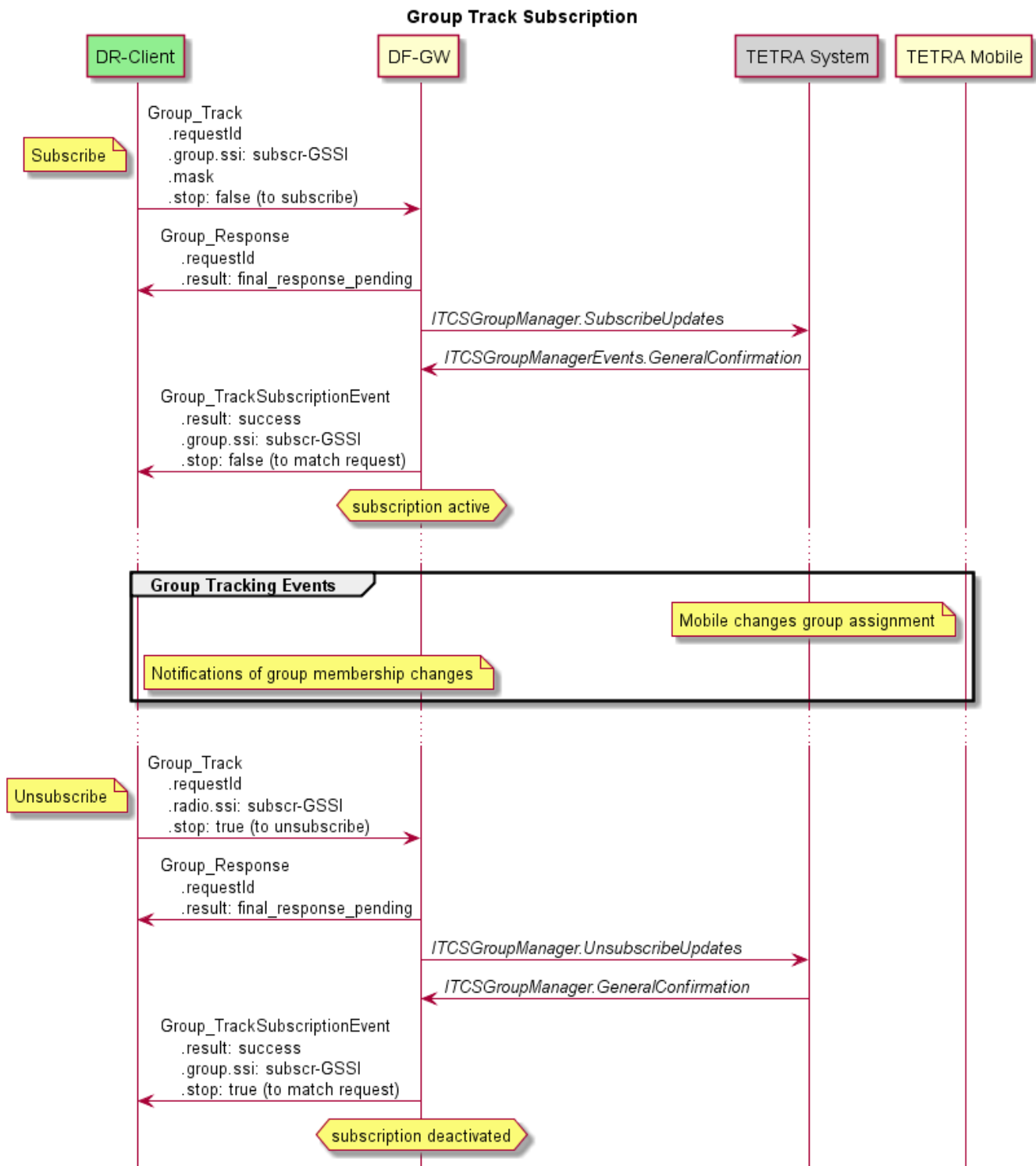
Figure 33 – Subscription for Group Tracking
