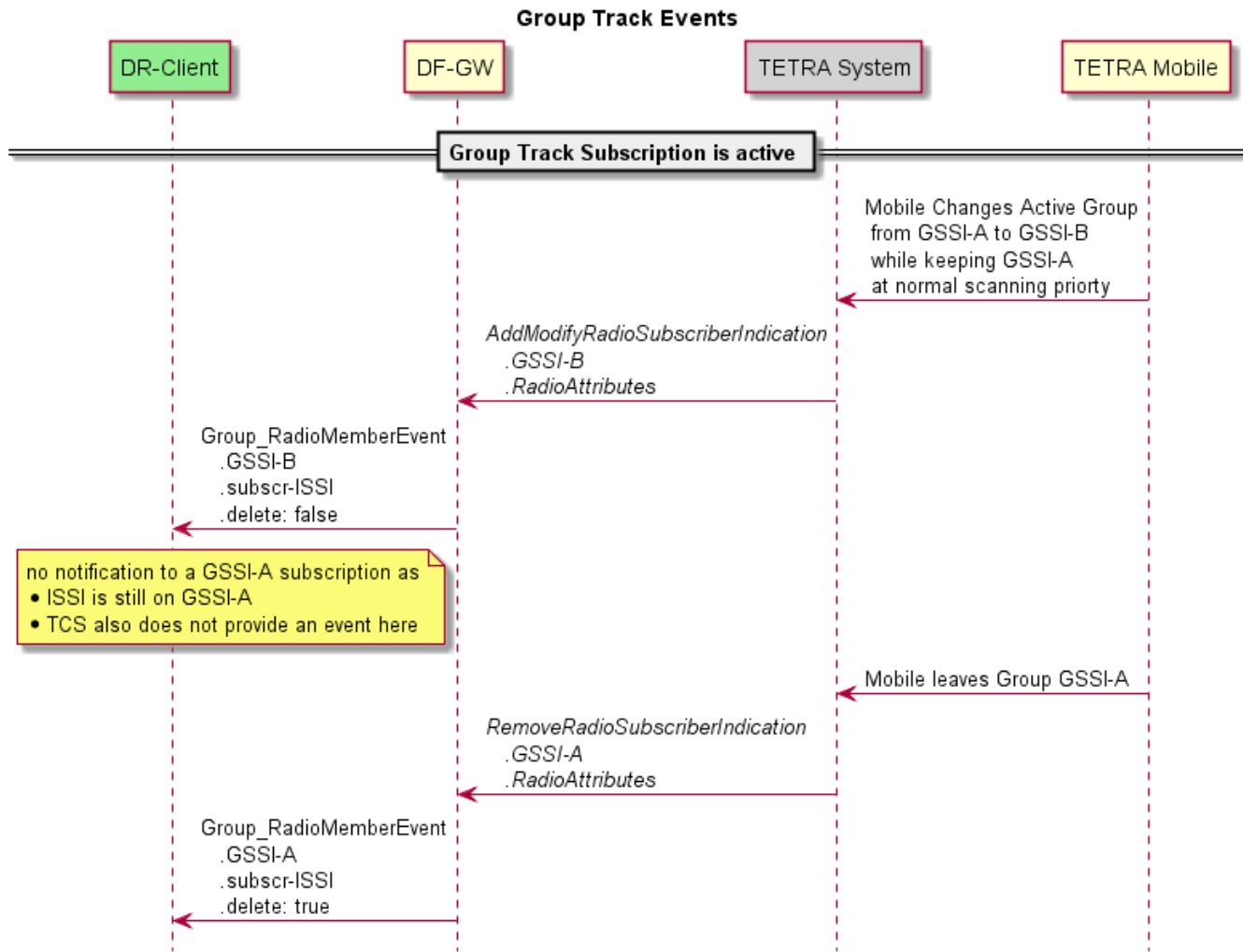
Figure 34 – Group Track Events
