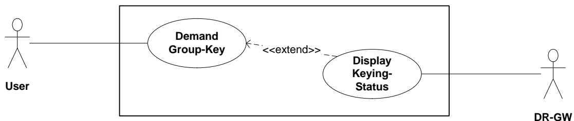
Figure 21 – Use Case Demanding a new key for a TETRA Group
