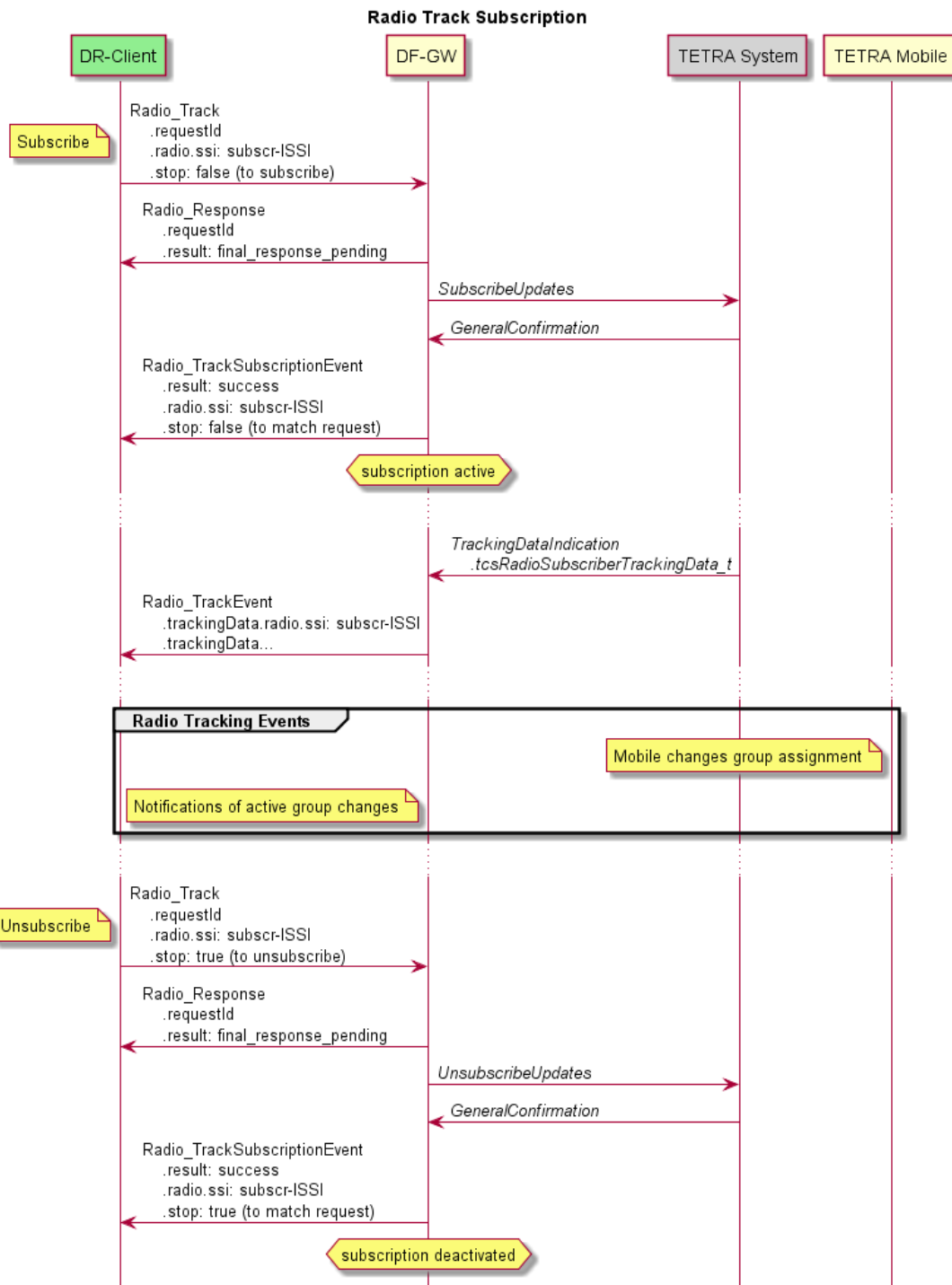
Figure 31 – Subscription for Radio Tracking
