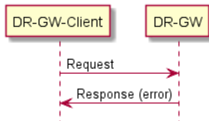
Figure 38 –Erroneous request
